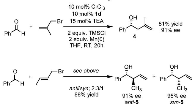
Scheme 1. Cr-Catalyzed Addition of Other Allylic Halides to Benzaldehyde
